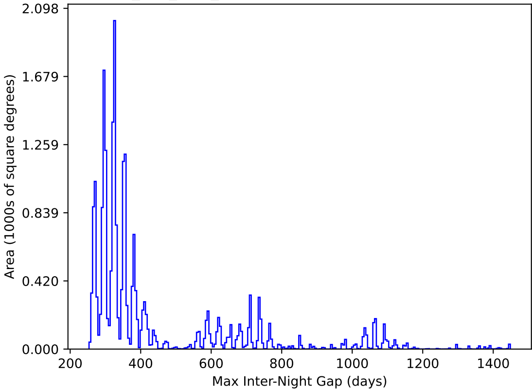
telescope_jerk_v3.5_10yrs All sky y band: Max Inter-Night Gap
