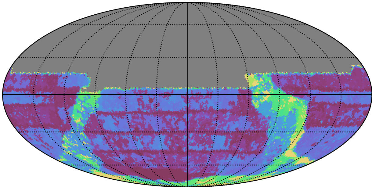
telescope_jerk_v3.5_10yrs All sky u band: Max Inter-Night Gap
