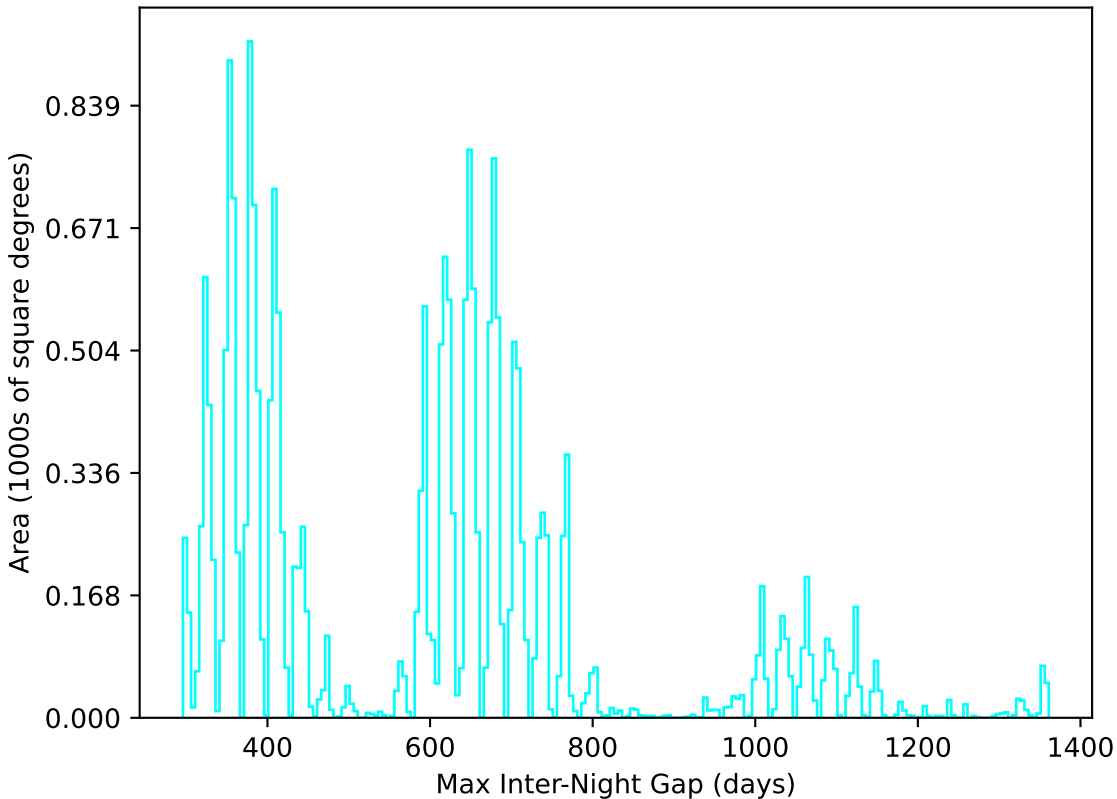
telescope_jerk_v3.5_10yrs All sky u band: Max Inter-Night Gap
