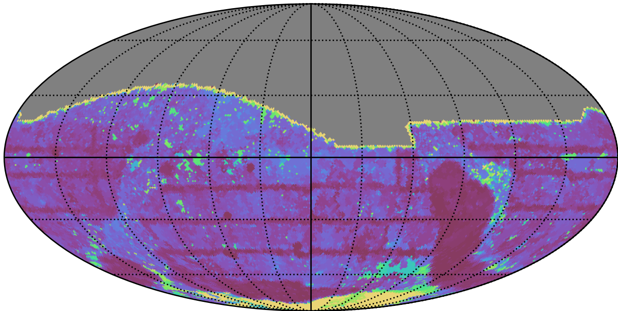
telescope_jerk_v3.5_10yrs All sky r band: Max Inter-Night Gap
