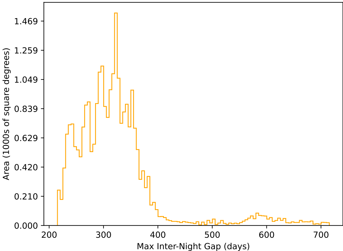
telescope_jerk_v3.5_10yrs All sky r band: Max Inter-Night Gap
