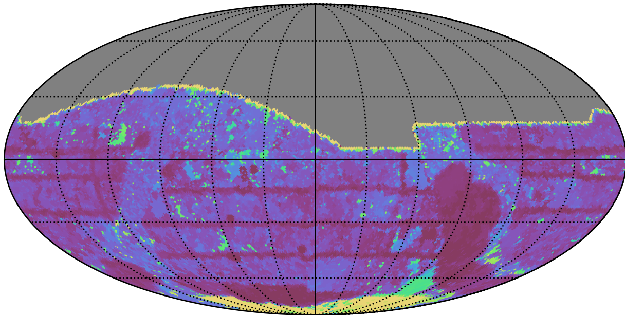
telescope_jerk_v3.5_10yrs All sky i band: Max Inter-Night Gap
