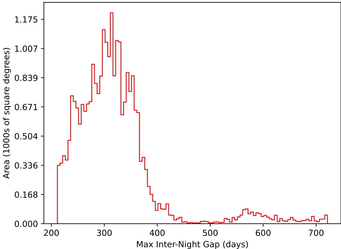
telescope_jerk_v3.5_10yrs All sky i band: Max Inter-Night Gap
