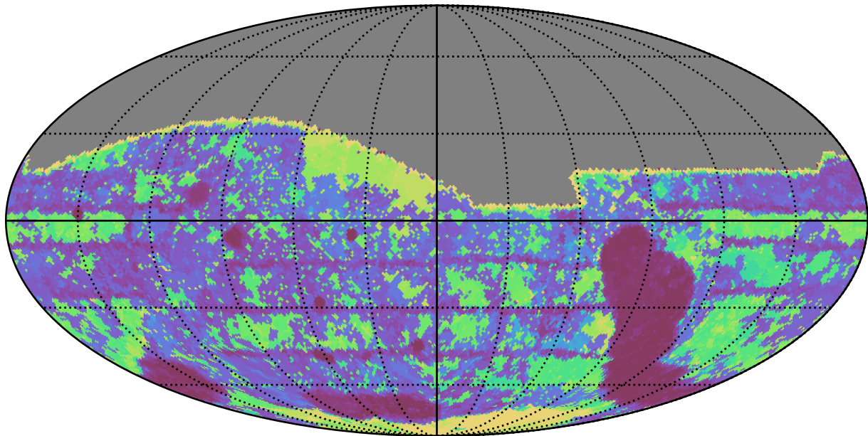
telescope_jerk_v3.5_10yrs All sky g band: Max Inter-Night Gap
