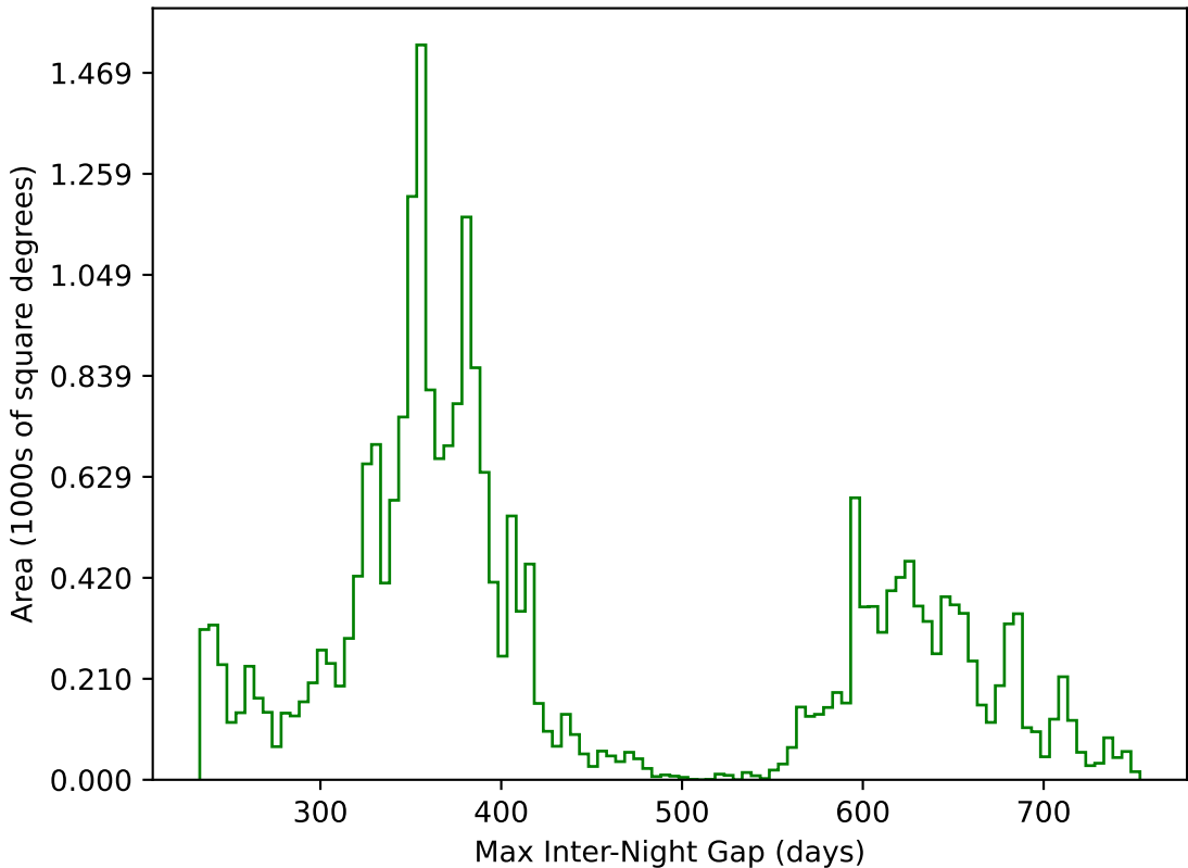
telescope_jerk_v3.5_10yrs All sky g band: Max Inter-Night Gap
