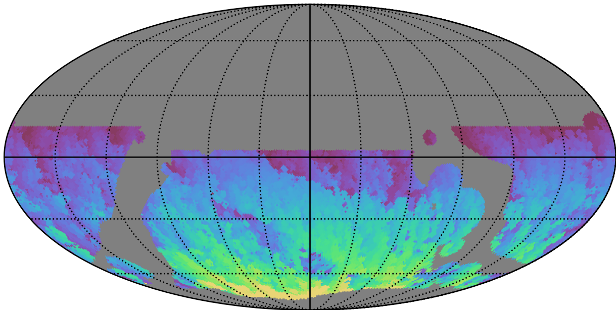
telescope_jerk_v3.5_10yrs WFD z band: Max HA
