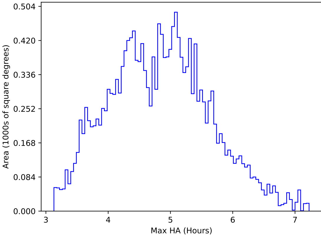
telescope_jerk_v3.5_10yrs WFD z band: Max HA
