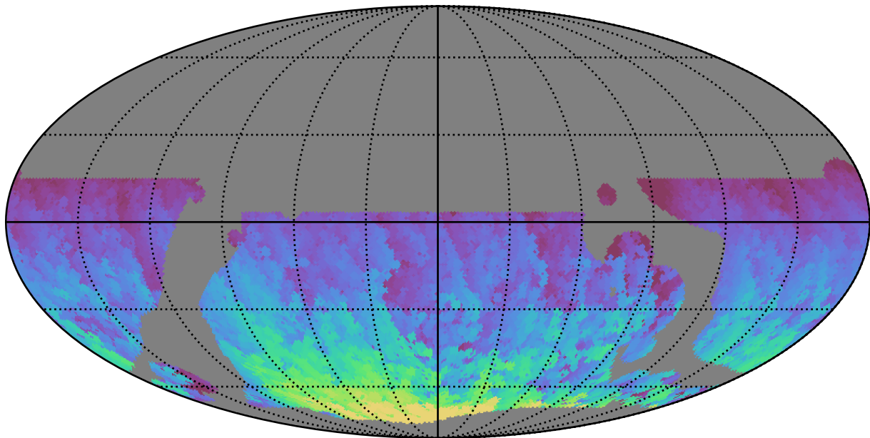
telescope_jerk_v3.5_10yrs WFD y band: Max HA
