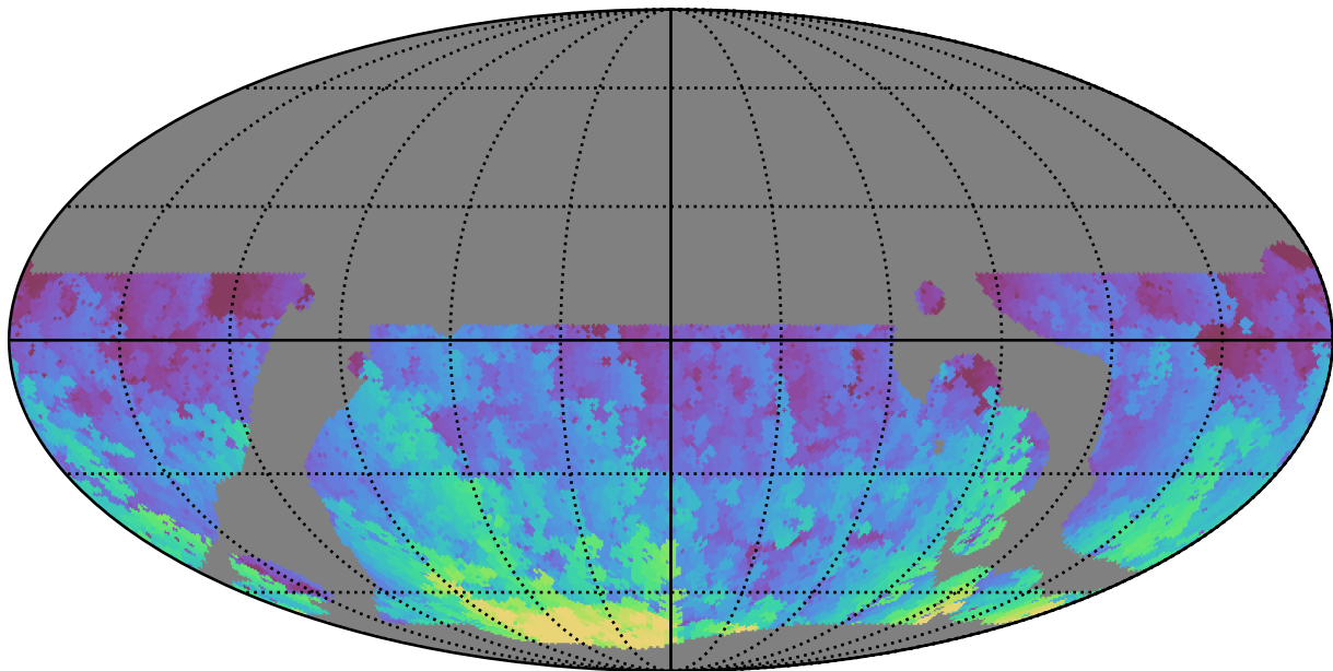
telescope_jerk_v3.5_10yrs WFD u band: Max HA
