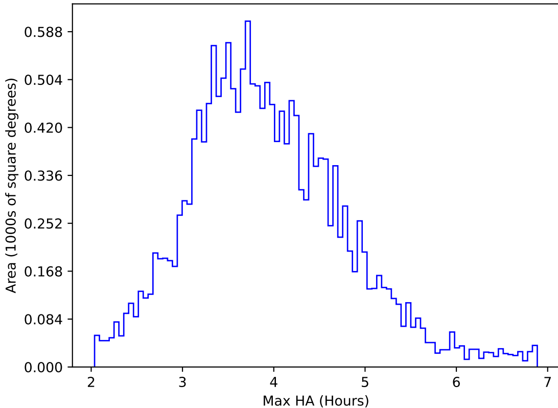
telescope_jerk_v3.5_10yrs WFD u band: Max HA
