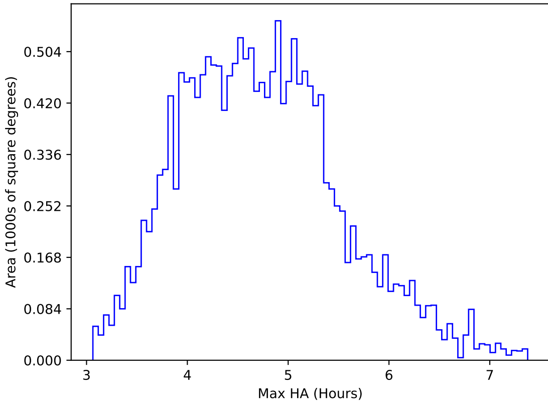
telescope_jerk_v3.5_10yrs WFD r band: Max HA
