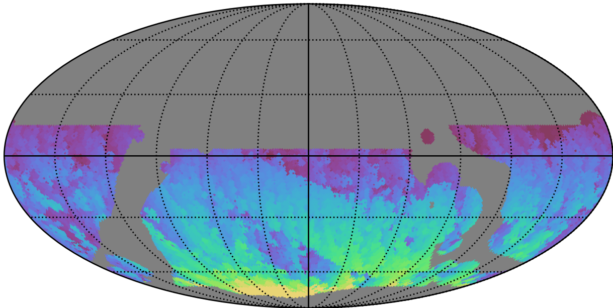
telescope_jerk_v3.5_10yrs WFD i band: Max HA
