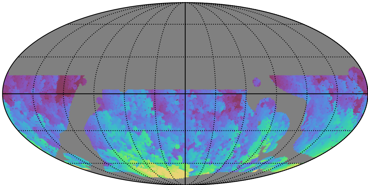
telescope_jerk_v3.5_10yrs WFD g band: Max HA
