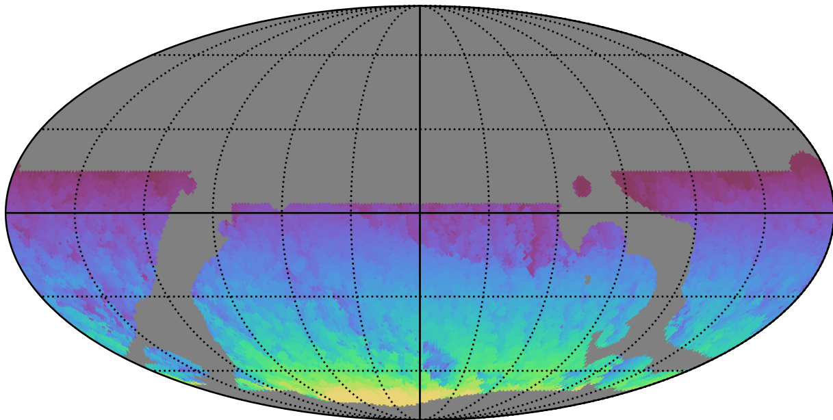
telescope_jerk_v3.5_10yrs WFD all bands: Max HA
