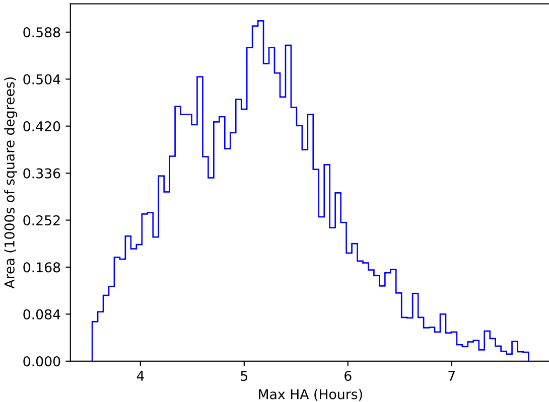
telescope_jerk_v3.5_10yrs WFD all bands: Max HA
