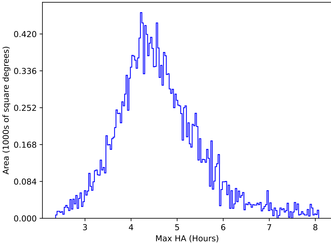
telescope_jerk_v3.5_10yrs All sky y band: Max HA
