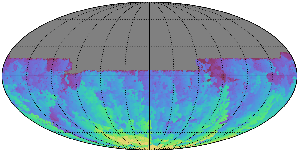
telescope_jerk_v3.5_10yrs All sky u band: Max HA
