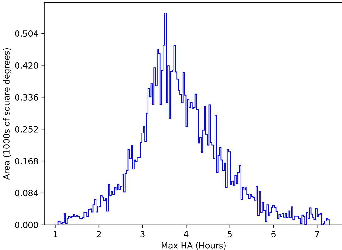
telescope_jerk_v3.5_10yrs All sky u band: Max HA
