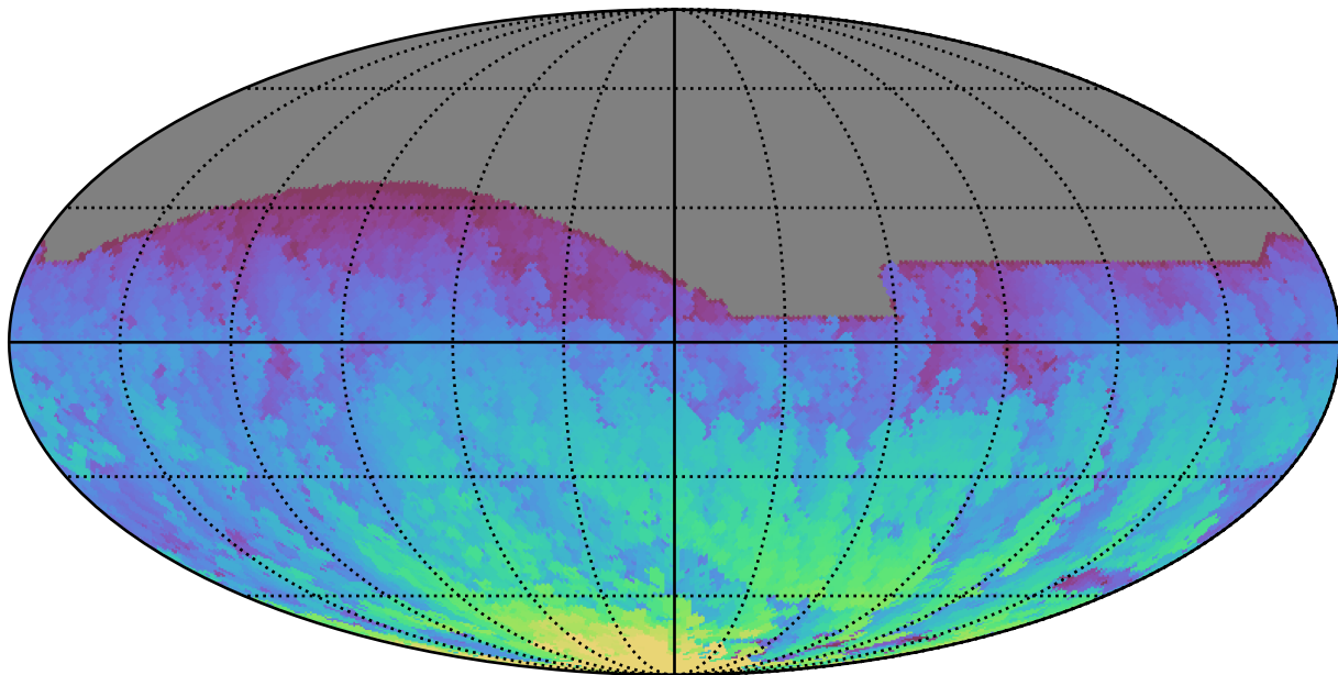
telescope_jerk_v3.5_10yrs All sky r band: Max HA
