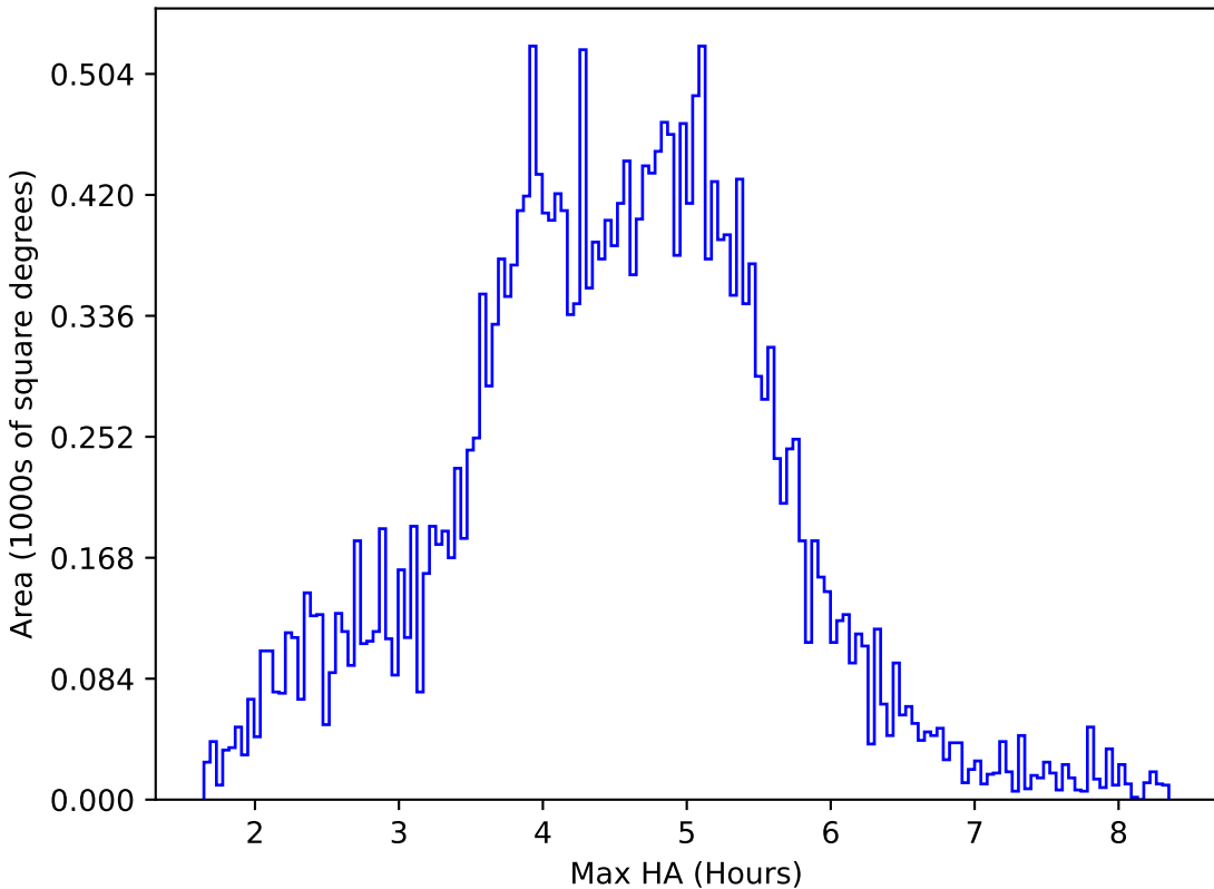
telescope_jerk_v3.5_10yrs All sky i band: Max HA
