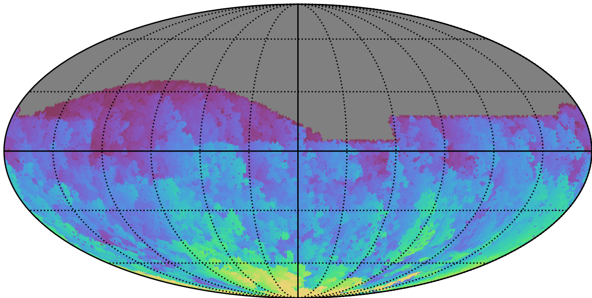
telescope_jerk_v3.5_10yrs All sky g band: Max HA
