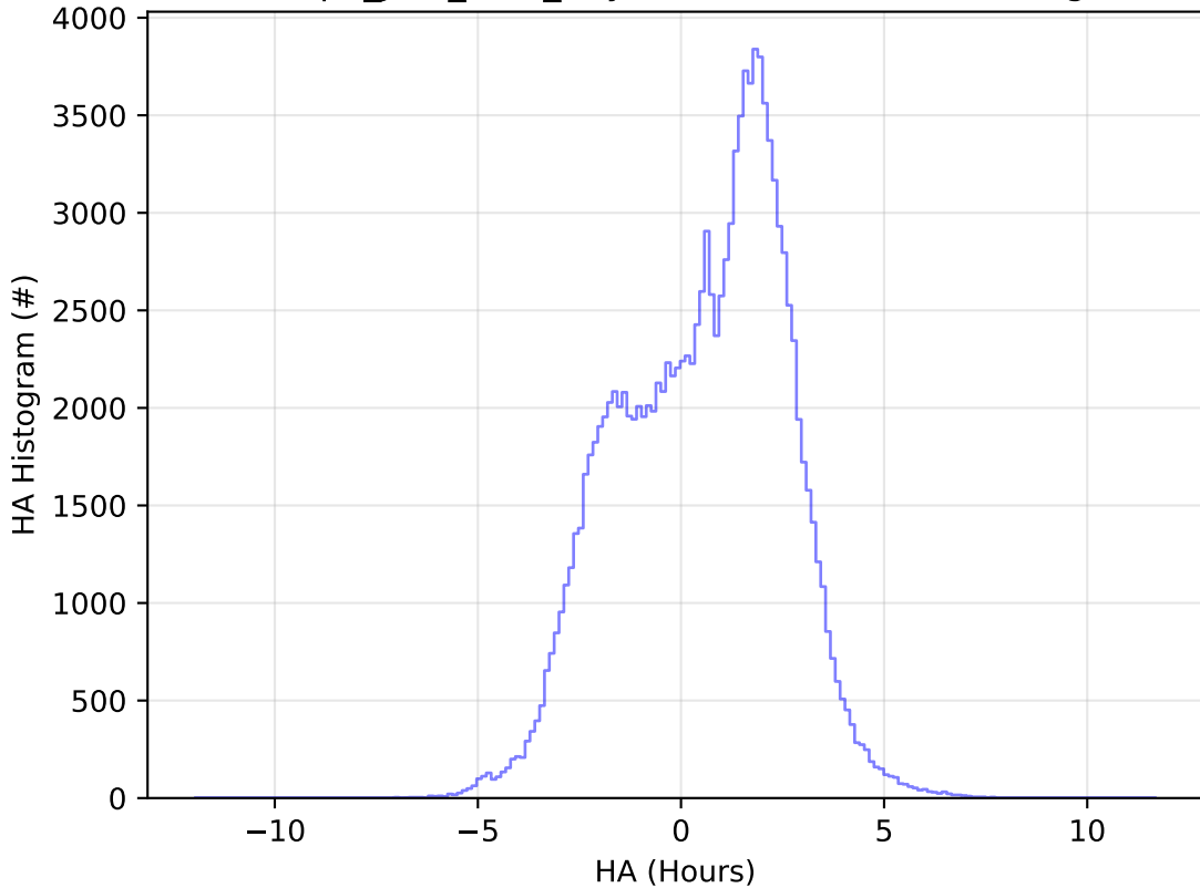
telescope_jerk_v3.5_10yrs WFD u band: HA Histogram
