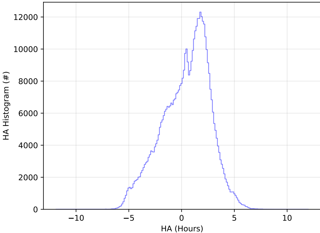
telescope_jerk_v3.5_10yrs WFD r band: HA Histogram
