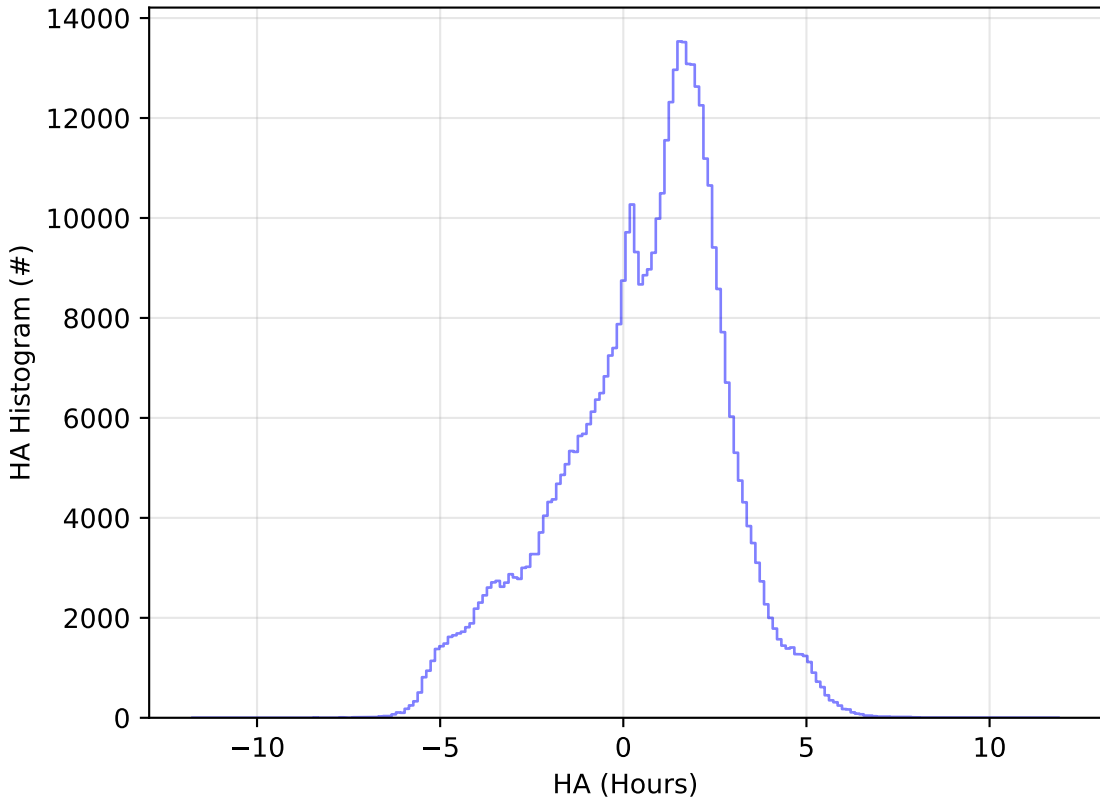
telescope_jerk_v3.5_10yrs WFD i band: HA Histogram
