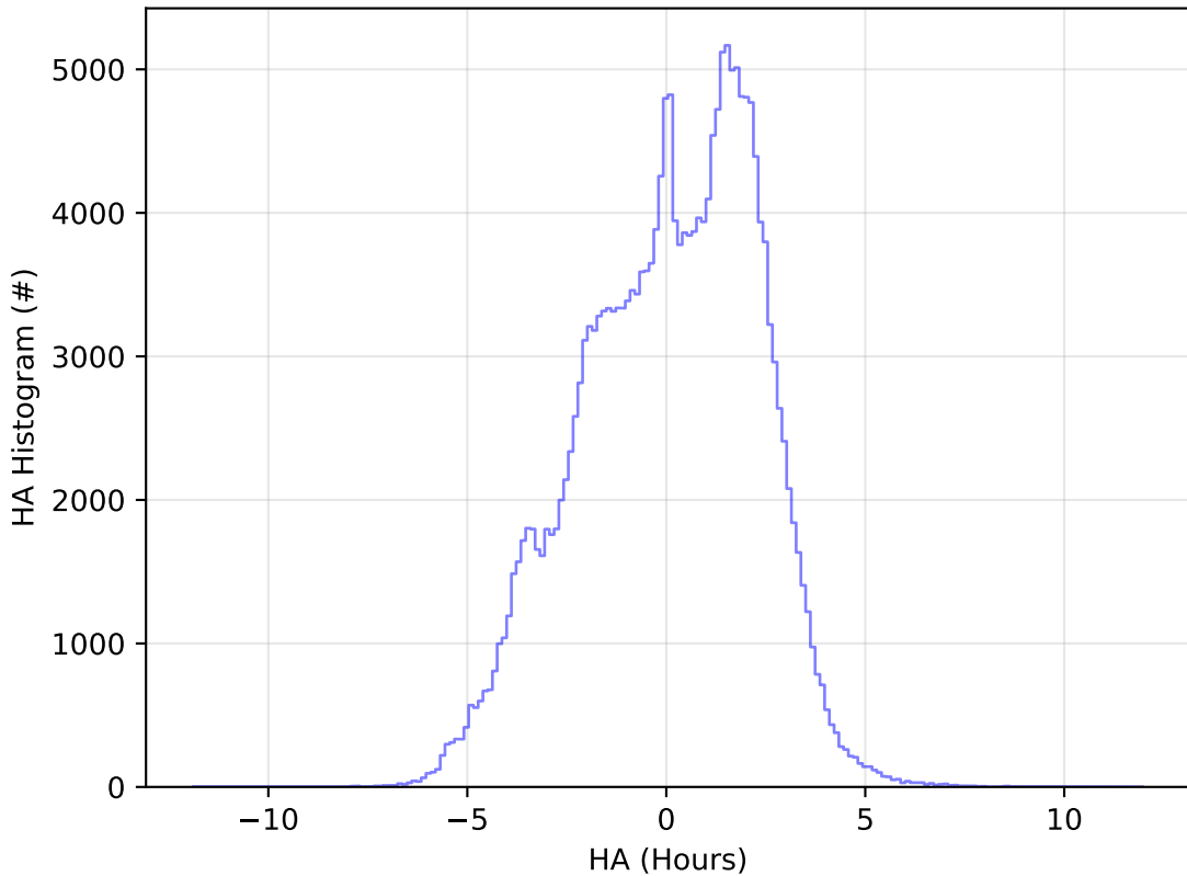
telescope_jerk_v3.5_10yrs WFD g band: HA Histogram
