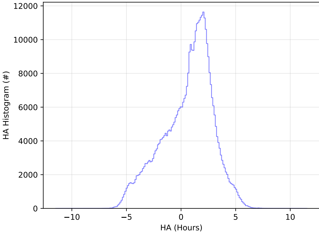
telescope_jerk_v3.5_10yrs All sky z band: HA Histogram
