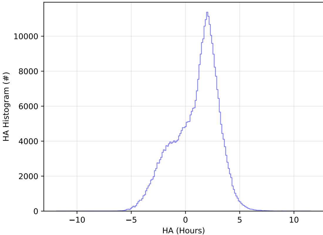
telescope_jerk_v3.5_10yrs All sky y band: HA Histogram
