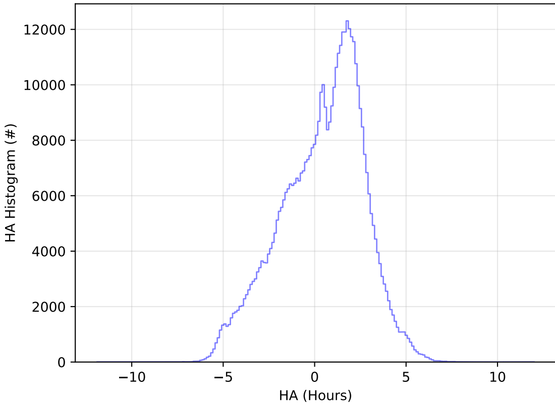
telescope_jerk_v3.5_10yrs All sky r band: HA Histogram
