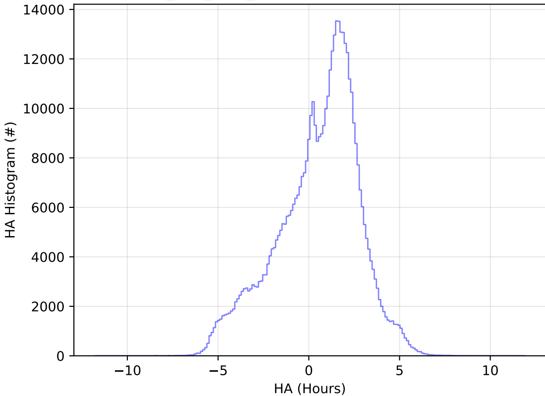
telescope_jerk_v3.5_10yrs All sky i band: HA Histogram
