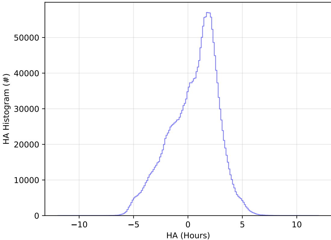
telescope_jerk_v3.5_10yrs All sky all bands: HA Histogram
