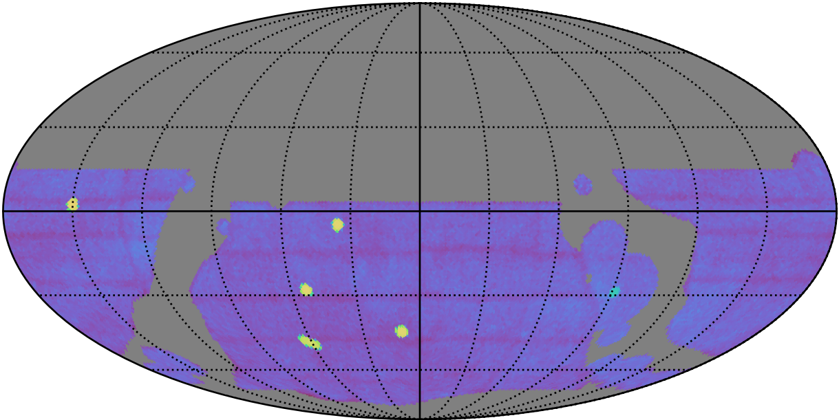
telescope_jerk_v3.5_10yrs gri WFD: Fraction of visits with a revisit < 60 min
