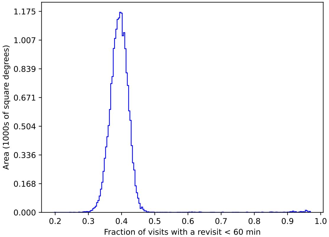
telescope_jerk_v3.5_10yrs gri WFD: Fraction of visits with a revisit < 60 min
