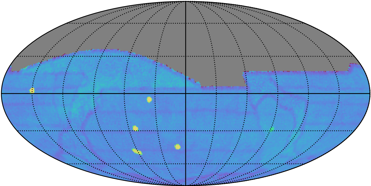
telescope_jerk_v3.5_10yrs gri All sky: Fraction of visits with a revisit < 60 min
