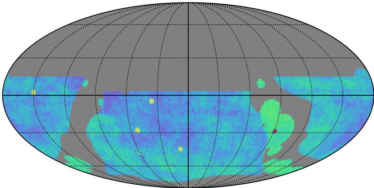
telescope_jerk_v3.5_10yrs gri WFD: Fraction of visits in pairs (20-90 min)
