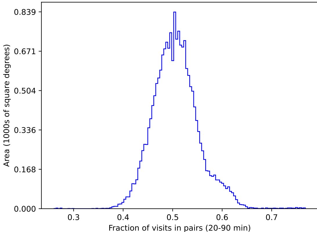
telescope_jerk_v3.5_10yrs gri WFD: Fraction of visits in pairs (20-90 min)
