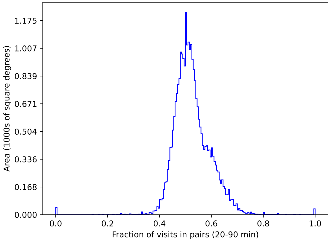
telescope_jerk_v3.5_10yrs gri All sky: Fraction of visits in pairs (20-90 min)
