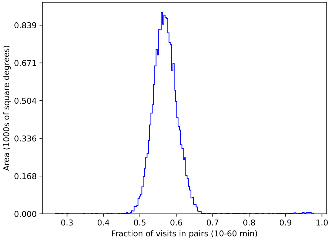
telescope_jerk_v3.5_10yrs gri WFD: Fraction of visits in pairs (10-60 min)
