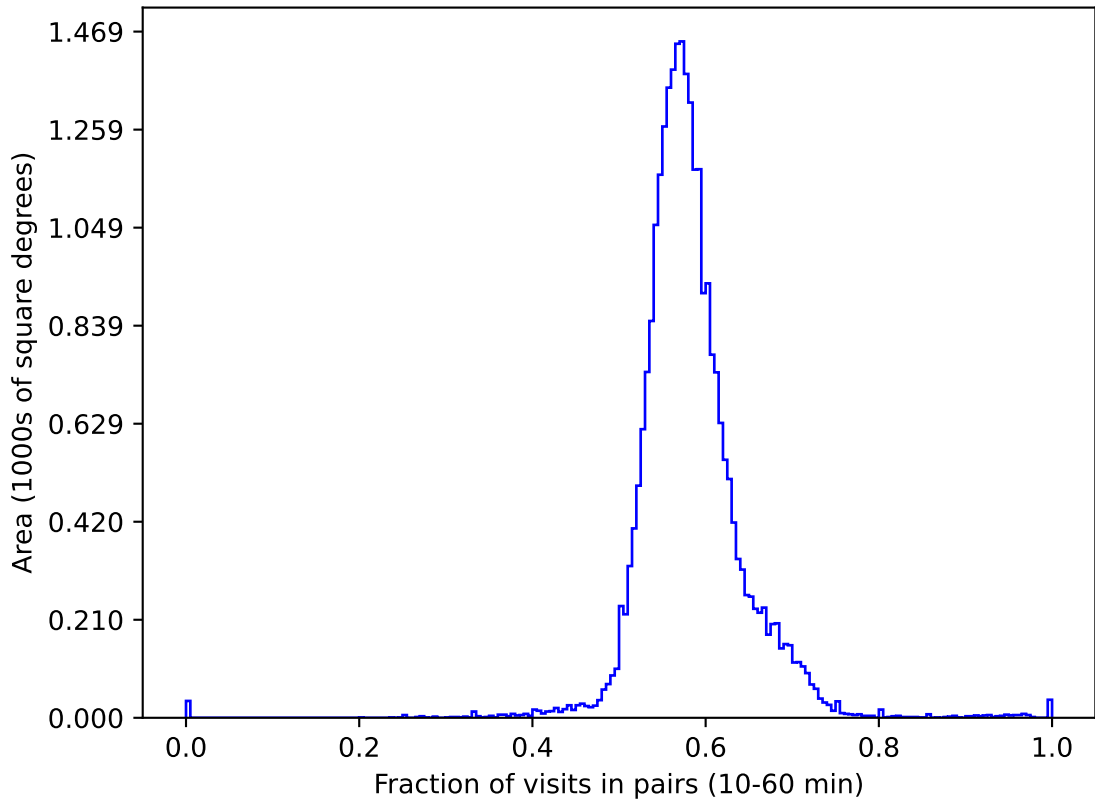
telescope_jerk_v3.5_10yrs gri All sky: Fraction of visits in pairs (10-60 min)
