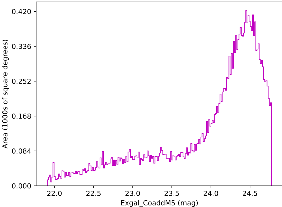
telescope_jerk_v3.5_10yrs Yr 3-4 z band: Exgal_CoaddM5
