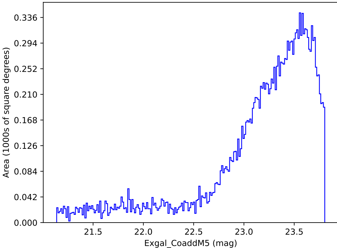
telescope_jerk_v3.5_10yrs Yr 3-4 y band: Exgal_CoaddM5
