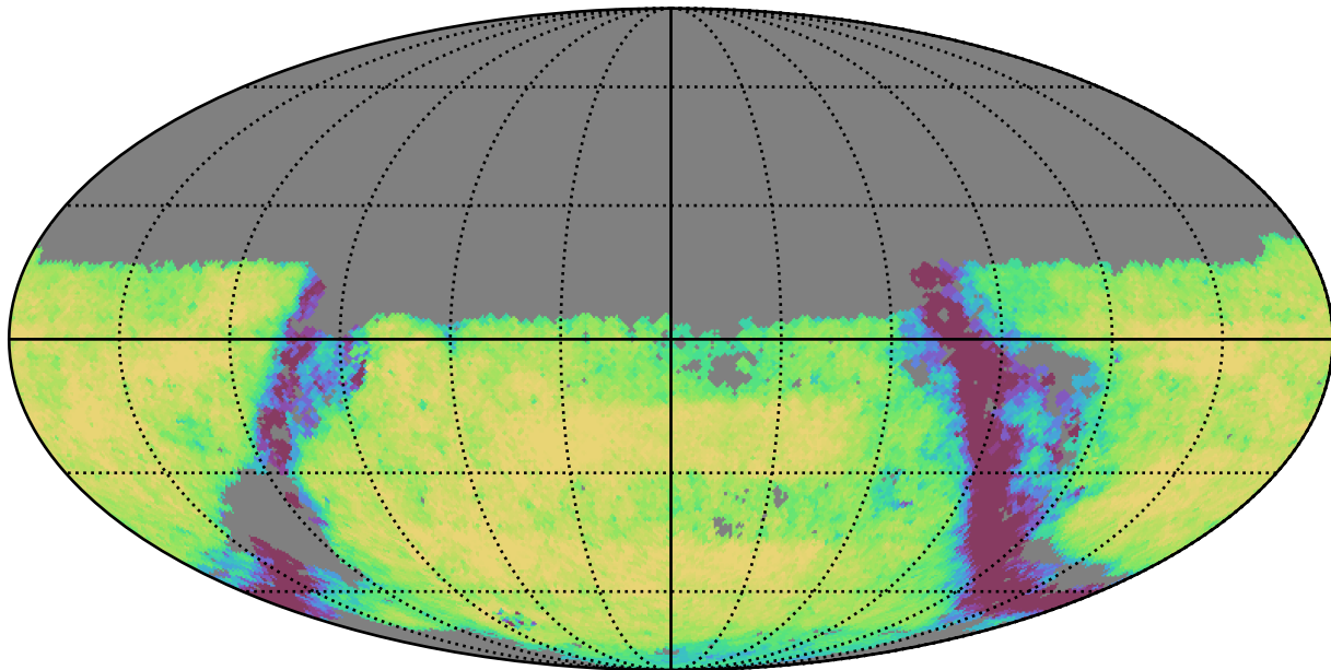
telescope_jerk_v3.5_10yrs Yr 3-4 u band: Exgal_CoaddM5
