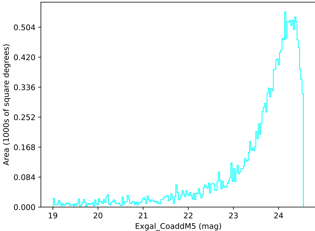
telescope_jerk_v3.5_10yrs Yr 3-4 u band: Exgal_CoaddM5
