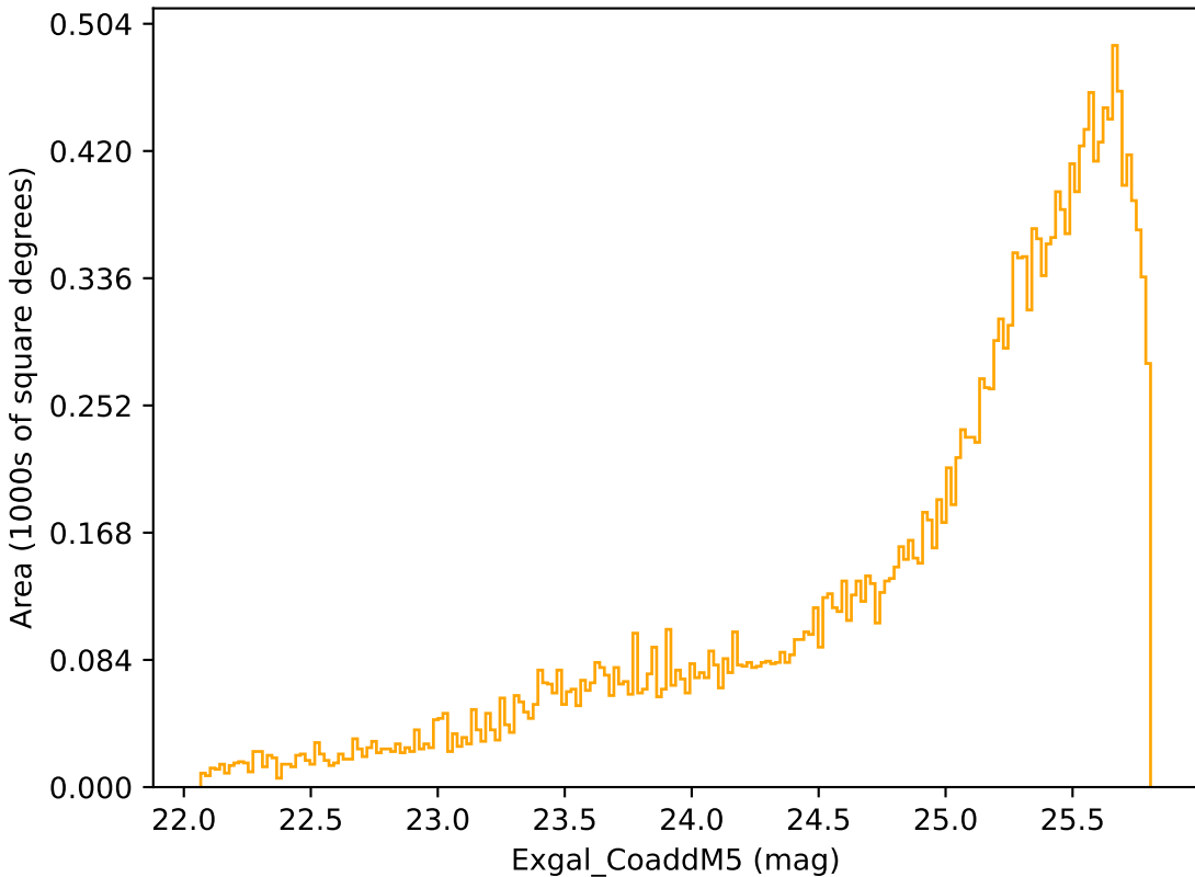
telescope_jerk_v3.5_10yrs Yr 3-4 r band: Exgal_CoaddM5
