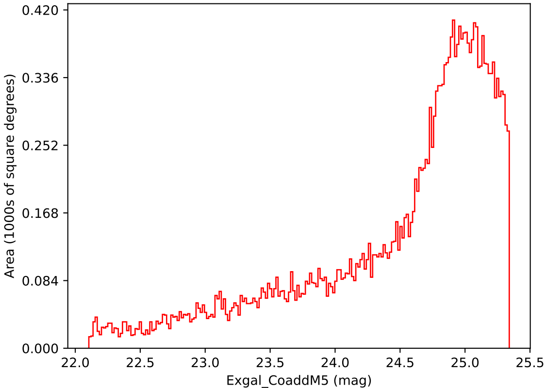
telescope_jerk_v3.5_10yrs Yr 3-4 i band: Exgal_CoaddM5
