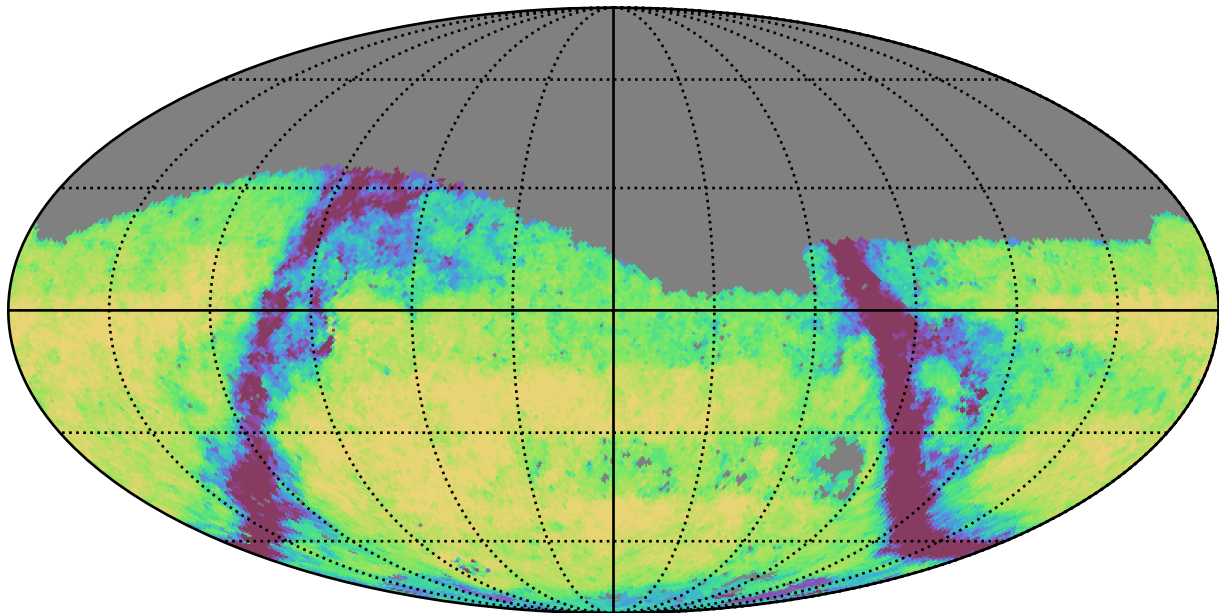
telescope_jerk_v3.5_10yrs Yr 3-4 g band: Exgal_CoaddM5
