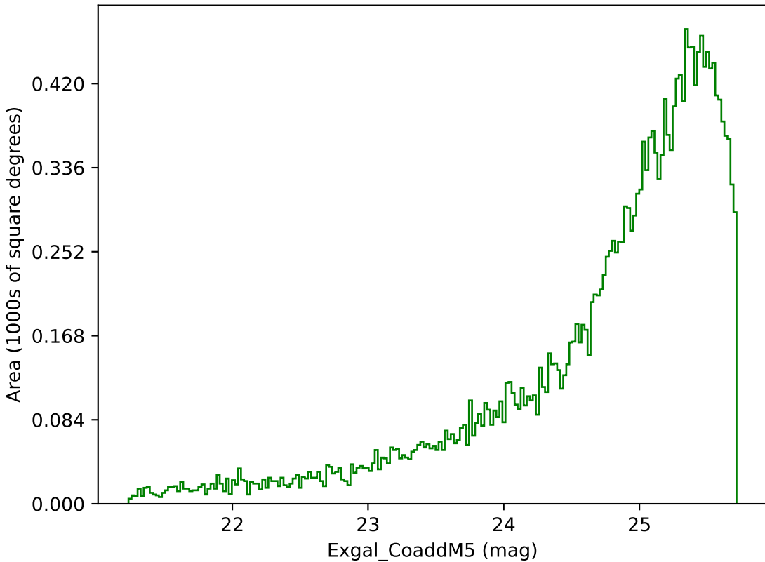
telescope_jerk_v3.5_10yrs Yr 3-4 g band: Exgal_CoaddM5
